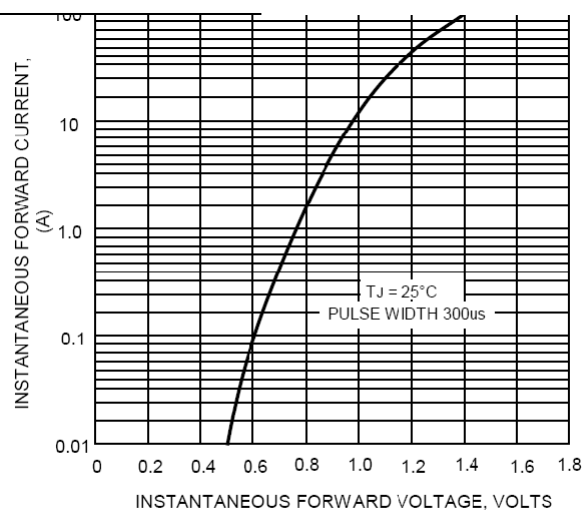
FIG.4-TYPICAL FORWARD CHARACTERISTICS
