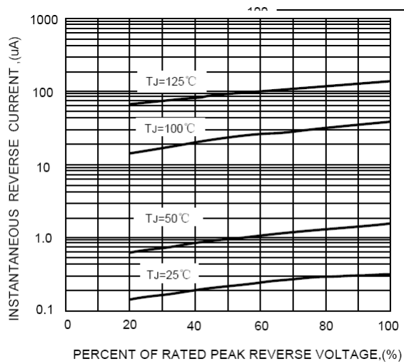
FIG.3-TYPICAL REVERSE CHARACTERISTICS
